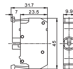
Contact block B3T...
