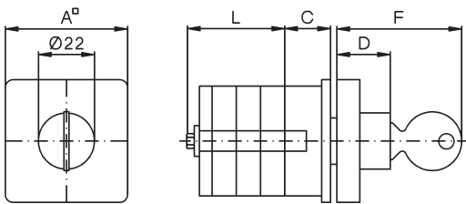
Key operated switch SAK Panel mounting E M10H, M10HD, M20
