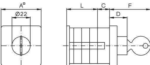
Key operated switch SAK Base mounting V M10H, M10HD, M20
