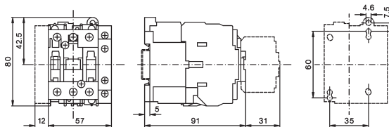
K3DC-20A10=, K3DC-48A10=
