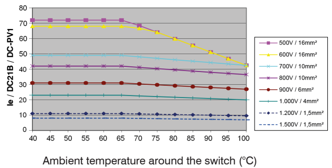
Switch open LS40 ..., 2 contacts in series + 2 parallel (A2+2)
