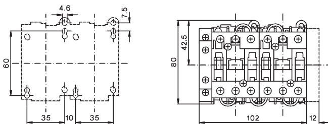
K3PV-100A00(=)
