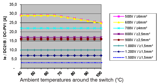
Switch open LS16 ..., 2 contacts in series + 2 parallel (A2+2)
