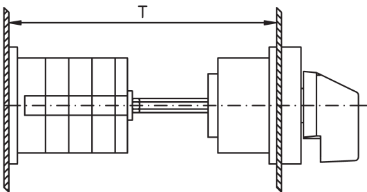
Door coupling, lockable TK2Z M10H, M10HD, M20, N20, N33F
