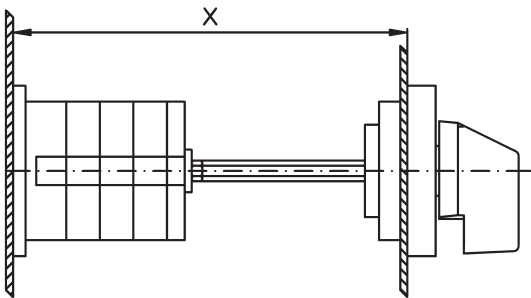
Door coupling, lockable TK2Z M10H, M10HD, M20, N20, N33F
