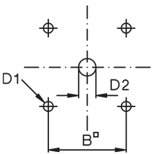
Mounting holes: TKZ
