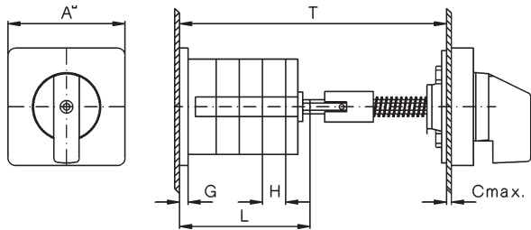
Door coupling TKE, TK2E M10H, M10HD, M20, N20, N33F
