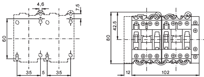
K3PV-30A10=, K3PV-60A10=
